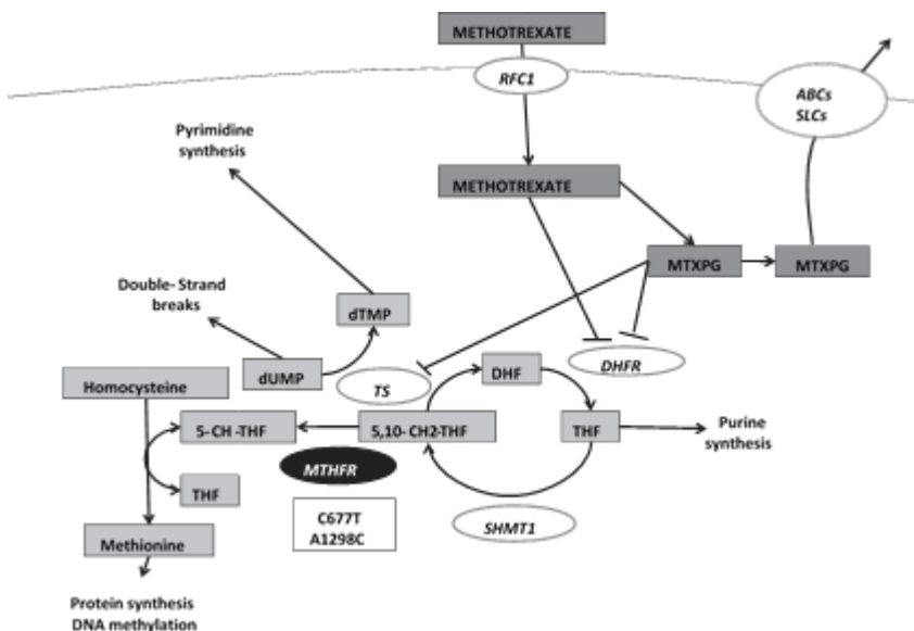
Figure 1. Folic acid metabolism and the effect of methotrexate (figure from Lopez-Lopez 2013).
